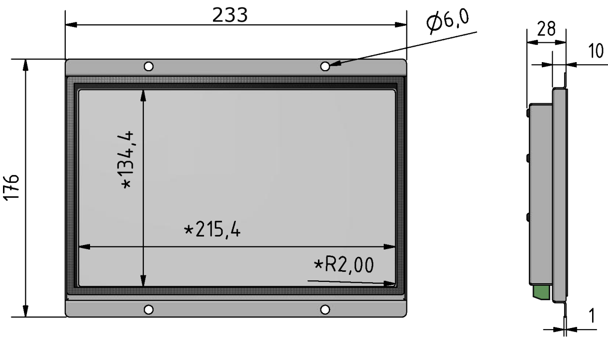
*Cutout front panel
