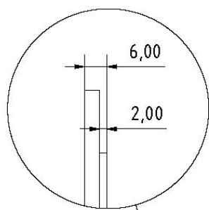
VSG safety glass 6 mm for 2 mm front panel
